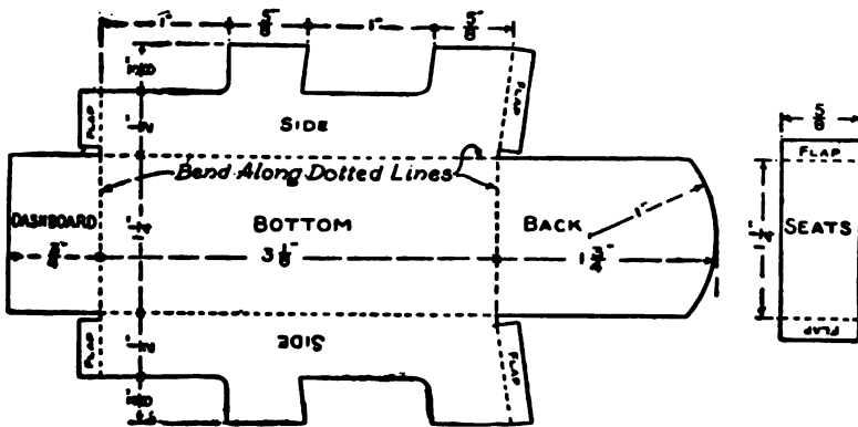
FIG. 144.—Pattern for the Merry-go-round Sleighs.
